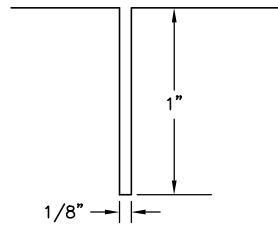
137 – TYPICAL SEASONAL SAWCUT
