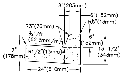
105 - B618 STANDARD CURB & GUTTER 105 - C&G (Bloom Std).dwg 5/2015
